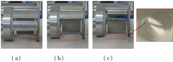
图 8 车轮从 (a)→(b)→(c) 滚动前进过程中的地面隆起现象 Fig.8 The phenomenon of ground swell as the wheel rolls from (a)→(b)→(c)
