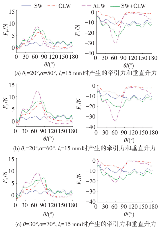
图 7 SW,CLW,ALW 以及 SW+CLW 产生的牵引力(左列)和垂直升力(右列)的比较 Fig.7 Comparison of drawbar pulls (left panels) and vertical forces (right panels) generated by the SW, the CLW, the ALW, and the sum of SW and CLW
